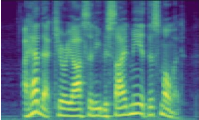
Spectrogram
