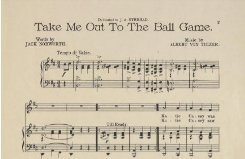
Sheet Music
